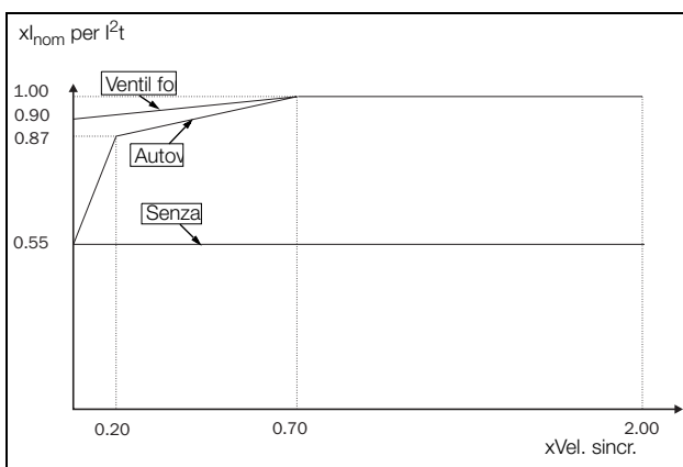
Fig. 92 Curve I^2t .
